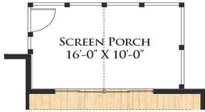
OPT GRILLE OR SCREENED PORCH
