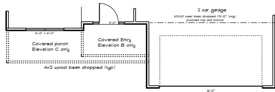
1st floor plan Elevation B & C
